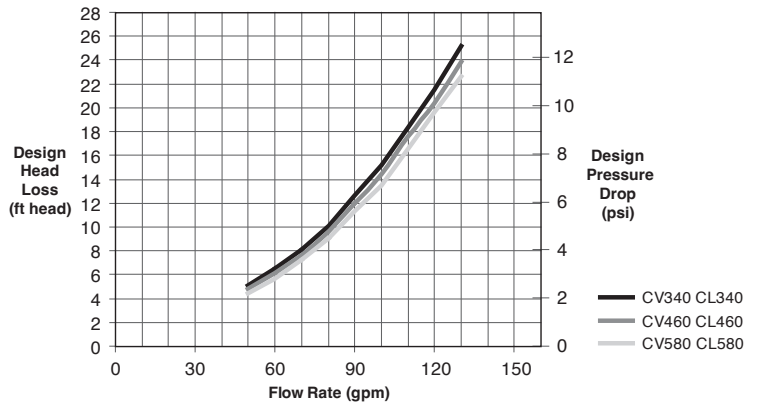
CV/CL Filter Head Loss Curves
